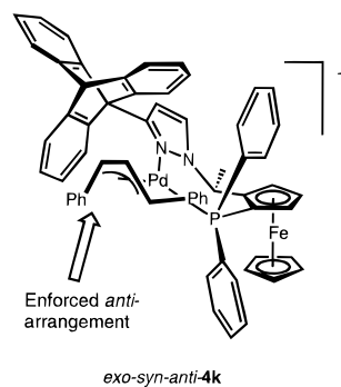
Figure 4. ORTEP view (20% ellipsoids) and atom numbering scheme for the cation ( R )-( S )- 4k .
