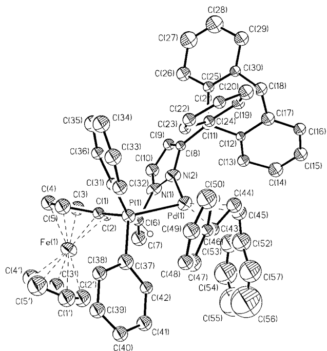
Figure 4. ORTEP view (20% ellipsoids) and atom numbering scheme for the cation ( R )-( S )- 4k .
